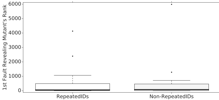
Fig. 33: CoREBench results on similar (repeatedIDs) and dissimilar (Non-RepeatedIDs) implementation. We observe similar trend in both cases suggesting a minor or no influence of code similarity on FaRM performance.
