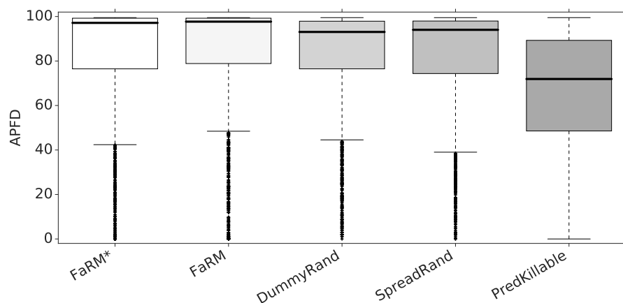
Fig. 17: APFD measurements considering all mutants for the selected mutants cost metric for Codeflaws. The FaRM prioritization outperform the random baselines.
