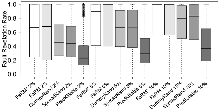
Fig. 11: Fault revelation of the mutant selection strategies on Codeflaws. All three FaRM and FaRM* sets outperform the random baselines.
