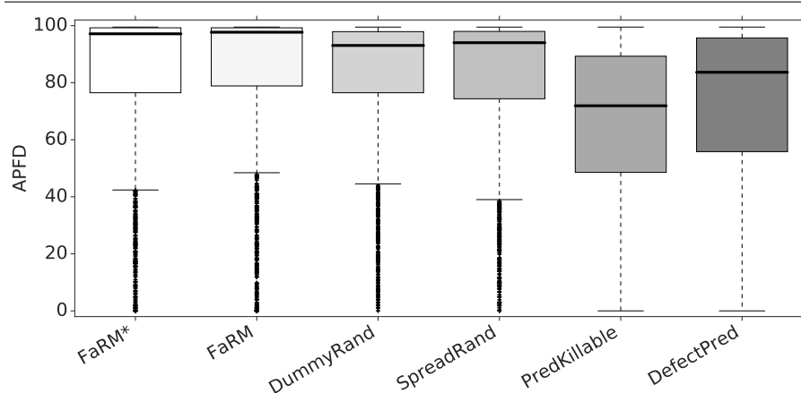
Fig. 23: APFD measurements considering all mutants. The FaRM prioritization outperform the defect prediction.
