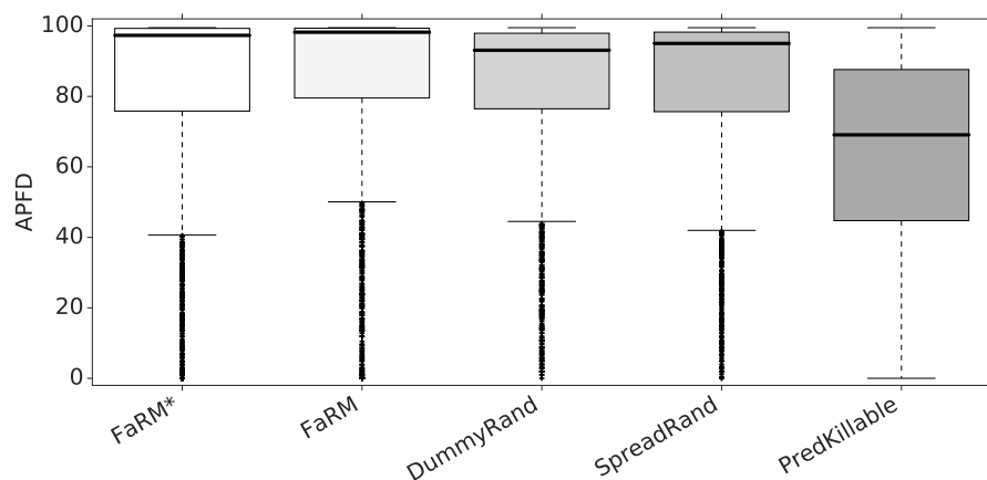
Fig. 18: APFD measurements considering only killable mutants for the selected mutants cost metric on Codeflaws. The FaRM prioritization outperform the random baselines, independent of non-killable mutants.
