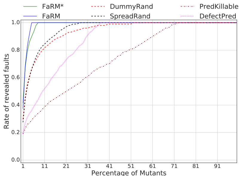
Fig. 24: Mutant prioritization performance in terms of faults revealed (median case) on CodeFlaws. The x-axis represent the number of considered mutants. The y-axis represent the ratio of the fault revealed by the strategies.
