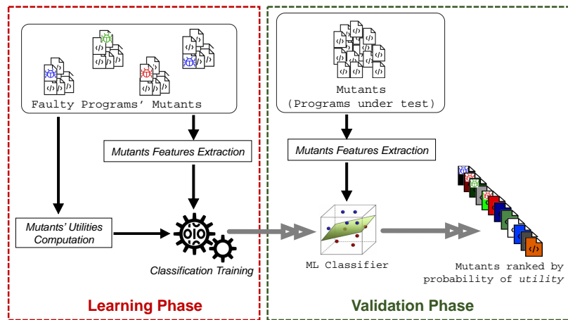
Fig. 2: Overview of the FaRM approach. Initially, FaRM applies supervised learning on the mutants generated from a corpus of faulty program versions, and builds a prediction model that learns the fault revealing mutant characteristics. This model is then used to predict the mutants that should be used to test other program versions. This means that at the time of testing and prior to any mutant execution, testers can use and focus only on the most important mutants.
