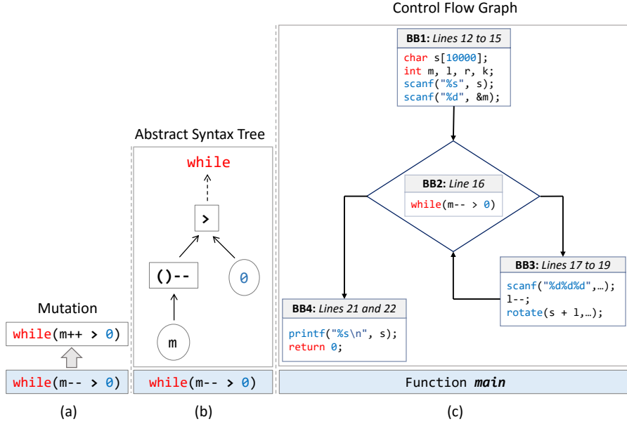
Fig. 5: (a) An example of mutant M from the example program from Figure 4, (b) the abstract syntax tree of the mutated statement and (c) the control flow graph of the function containing the mutated statement.
