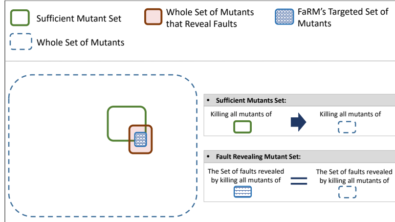
Fig. 1: Fault revealing mutant selection. Contrast between sufficient mutant set selection and fault revealing mutant selection. Sufficient mutant set selection aims at selecting a minimal subset of mutants that is killed by tests that also kill the whole set of mutants. Fault revealing mutant selection aims at selecting a minimal subset of mutants that is killed by tests that reveal the same underlying faults as the tests that kill the whole set of mutants.
