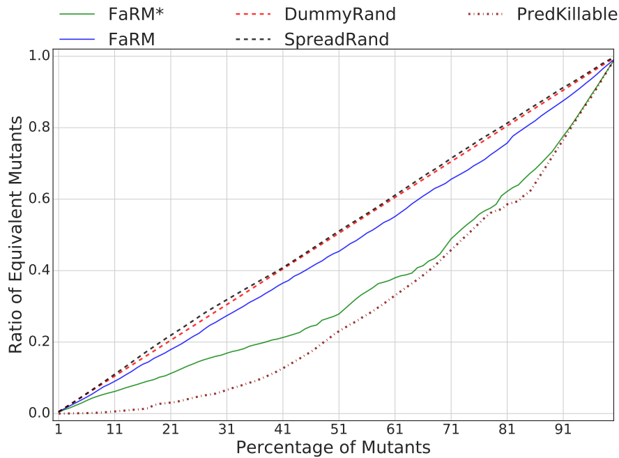
Fig. 29: Ratio of equivalents (median case) on CoREBench. The x-axis represent the number of considered mutants, while the y-axis represent the proportion of equivalent mutants selected by the strategies.
