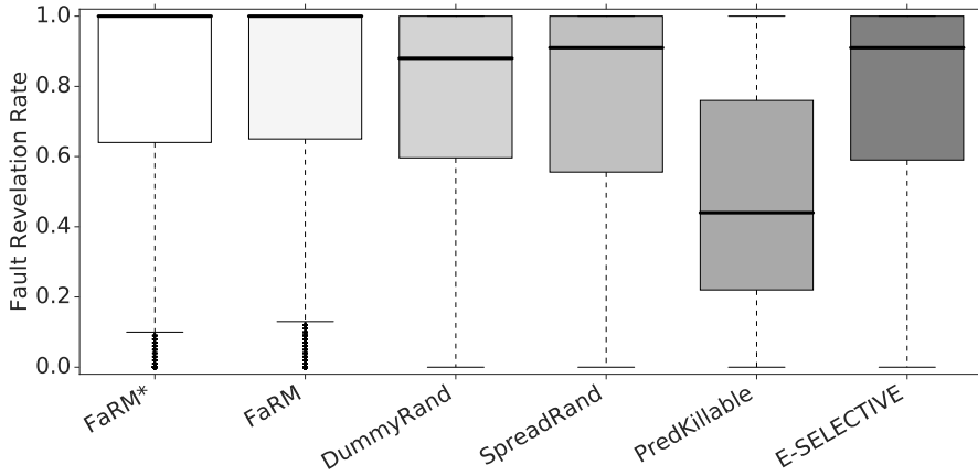
Fig. 16: Fault revelation of FaRM compared with E-Selective for selection size 15% of all mutants. FaRM sets outperform E-Selective selection.
