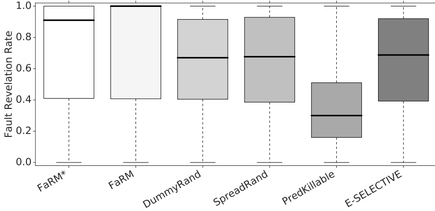
Fig. 14: Fault revelation of FaRM compared with E-Selective on Codeflaws. Approximately 38% (number of E-Selective mutants) of all the mutants are selected.
