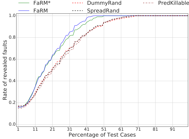
Fig. 22: Required tests prioritization performance in terms of faults revealed (median case) on CodeFlaws. The x-axis represent the number of considered tests. The y-axis represent the ratio of the fault revealed by the strategies.
