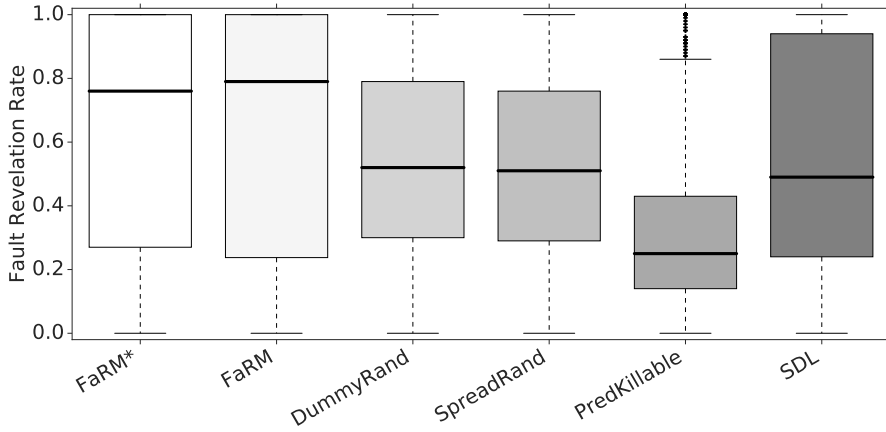
Fig. 13: Fault revelation of FaRM compared with SDL on Codeflaws. FaRM sets outperform the SDL selection. Approximately 2% (number of SDL mutants) of all the mutants are selected.
