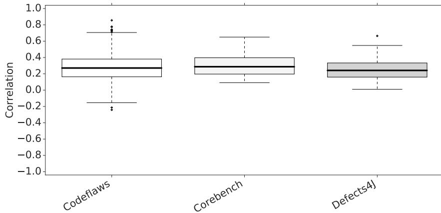
Fig. 32: Correlations between mutants and faults in three defect datasets. Similar correlations are observed in all three cases suggesting that Codeflaws provides good indications on the fault revealing ability of the mutants.
